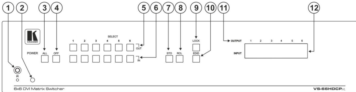
Figure 1: VS-66HDCPxL 6x6 DVI Matrix Switcher Front Panel
