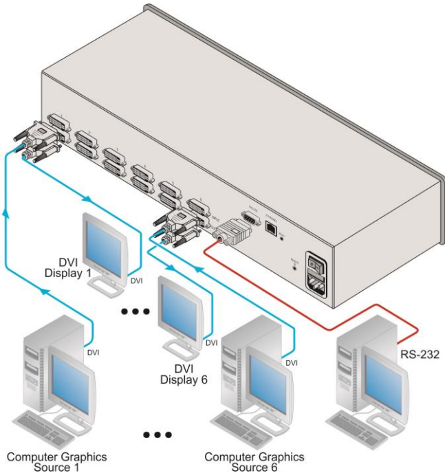
Figure 3: Connecting the VS-66HDCPxI 6x6 DVI Matrix Switcher
