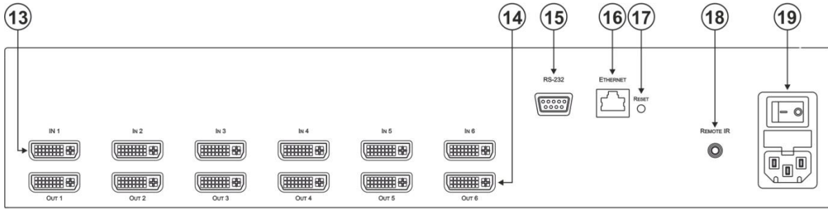
Figure 2: VS-66HDCPxI 6x6 DVI Matrix Switcher Rear Panel
