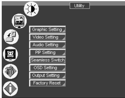
Figure 27: Utility Screen
