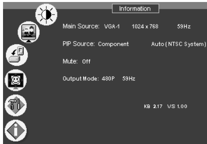
Figure 48: Information Screen
