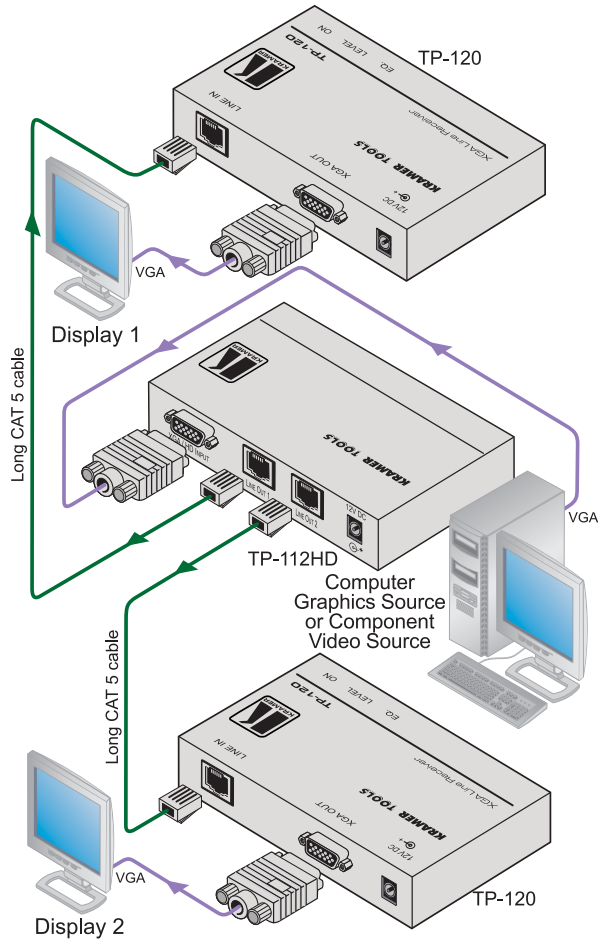
Figure 5: Configuring a 1:2 XGA/HD to Twisted Pair Transmitter/Receiver/DA
