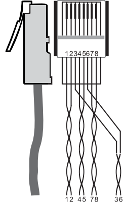
Figure 6: CAT 5 PINOUT
