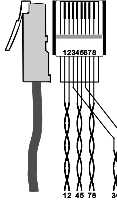
Figure 4: CAT 5 PINOUT
