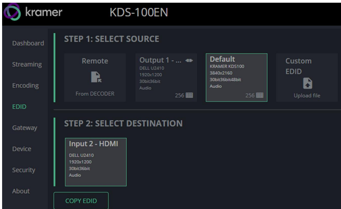
Figure 17: EDID pane
