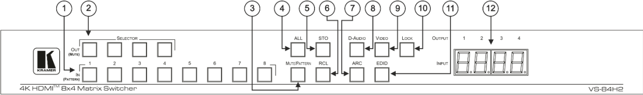
Figure 3: VS-84H2 8x4 Matrix Switcher Front Panel
