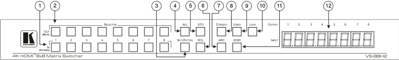
Figure 1: VS-88H2 8x8 4K60 HDMI Matrix Front Panel
