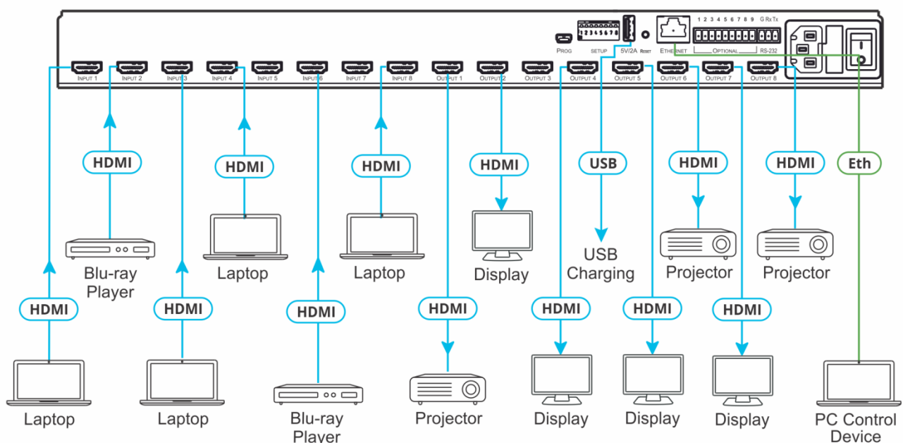
Figure 7: Connecting to the VS-88H2 Rear Panel
