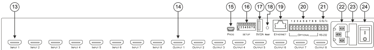
Figure 4: VS-88H2 8x8 4K60 HDMI Matrix Rear Panel
