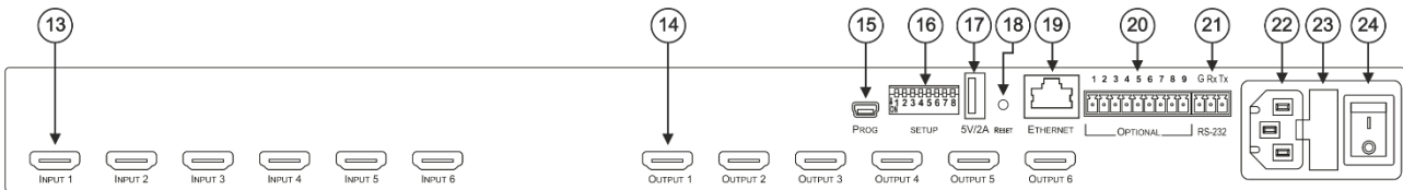
Figure 5: VS-66H2 6x6 Matrix Switcher Rear Panel
