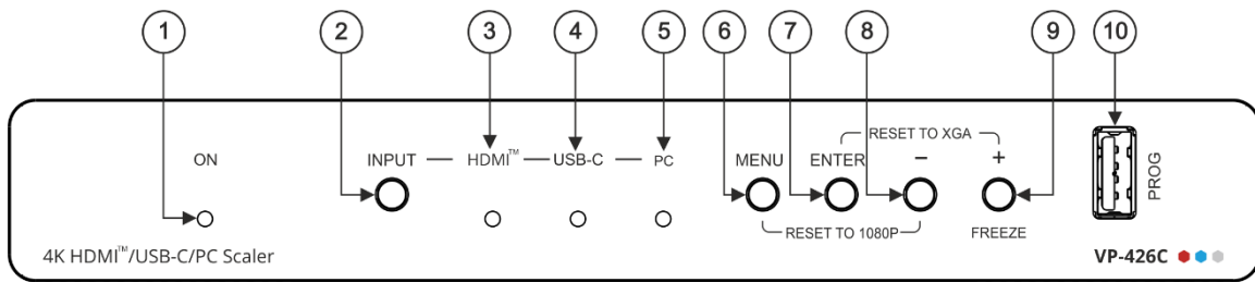
Figure 1: VP-426C 4K HDMI/USB-C/PC Scaler Front Panel
