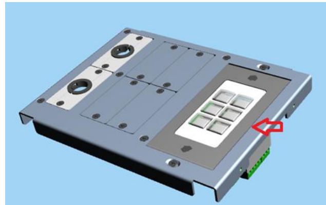
Figure 2: Control Panel Installed in TBUS Using T-1GD
